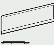
300.FP.45.06 W 25 3/16" 300.FP.45.07 W 31 1/8" 300.FP.45.09 W 39" 300.FP.45.11 W 46 7/8" 300.FP.45.13 W 54 3/4" 300.FP.45.15 W 62 5/8" 300.FP.45.17 W 70 1/2" Frontal panel per profilo attrezzabile DV801 / Frontal panel for accessories profile DV801
