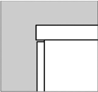
E23 SQUARE EDGE 1.25" AVAILABLE ON TOP SURFACE ONLY 1.5" AVAILABLE ON OVERLAY RUNOFFS ONLY
