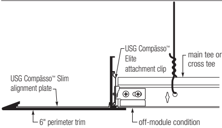
B. Edge Detail – USG Donn® Brand DX®/DXL™ and Centricitee™, Full and Partial Module
