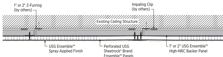
Direct Mount Z-Furring System
