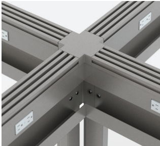
X-Connector
