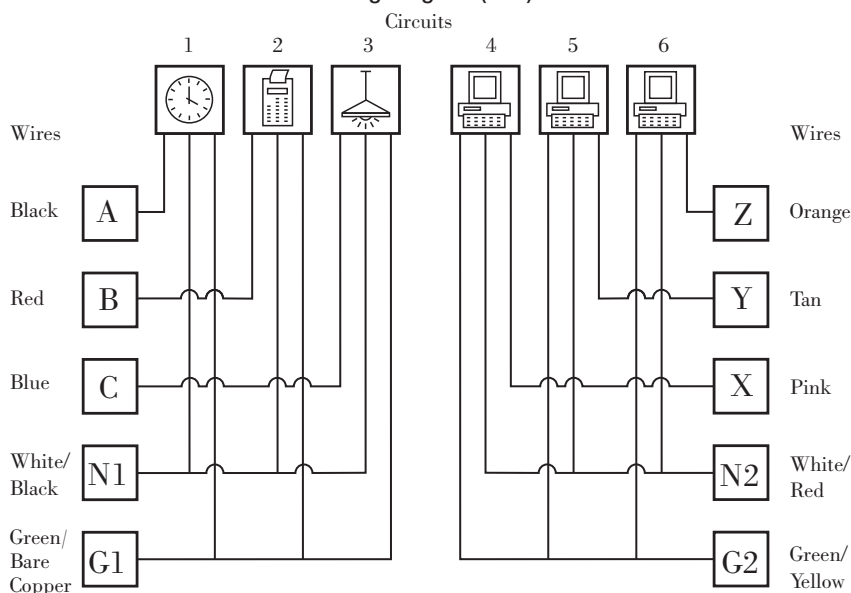
Wiring Diagram (3+3)
