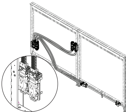
Double Vertical Electrical within Same Frame
