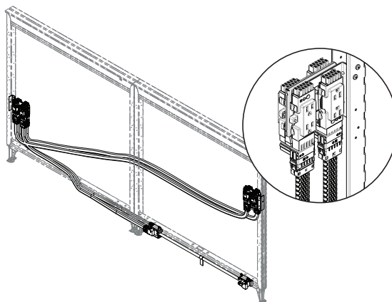
Double Vertical Electrical within Adjacent Frame
