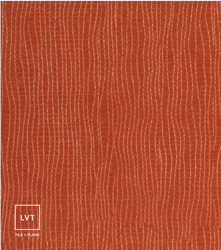
SUBSTRATE, MAGMA
