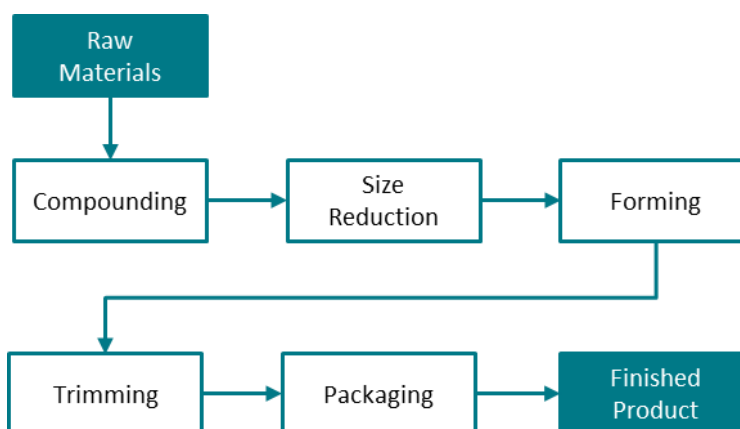
Figure 2: Diagram of production process – heterogeneous vinyl flooring
