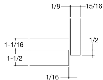
DETAIL B OVERHEAD w/ HINGED DOOR
