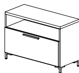
Credenza Open/File W: 18, 24, 30, 36, 42 D: 16, 20 H: 25 Keyless Locking Available 30" w and larger
