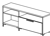
Credenza Box/File W: 18, 24, 30, 36, 42 D: 16, 20 H: 25 Keyless Locking Available 30" w and larger
