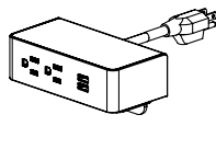
Desktop Power Module, 3-Prong Plug 2 Duplexes + 2 USB Braided or Standard Cordset Cord Length: 36, 72
