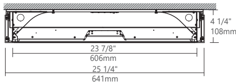
SECTION VIEW
