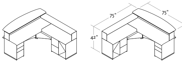
1030 - 40 Parabola Reception Desk with gallery radius front and L-shaped return Desk with one pedestal, radius front w 75" d 36" h 42" Return with gallery wall and double pedestal, straight front w 75" d 23" h 42"
