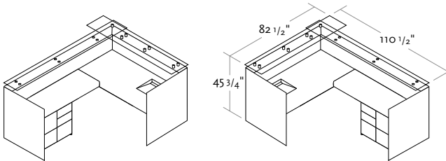
25100 Reception Desk with gallery surround glass transaction top and straight front w 110 1/2" d 82 1/2" h 45 3/4"
