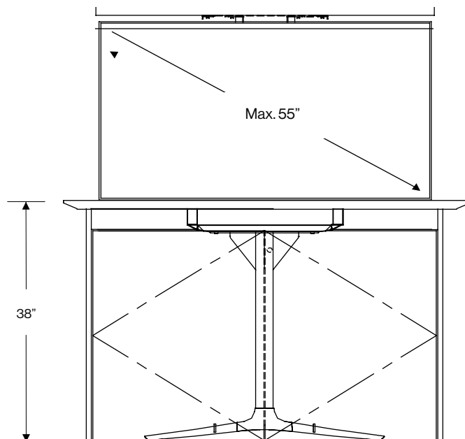
Elevation for 38"h Media Lift Table
