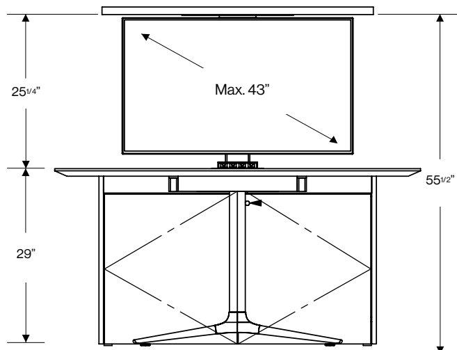
Elevation for 29"h Media Lift Table
