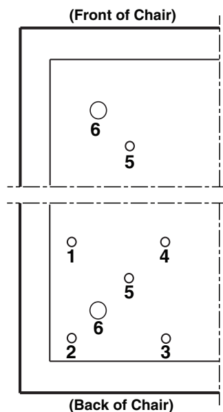
JENNY CLUB LOW HOLE TEMPLATE (Typical Front and Back Corners)
