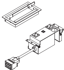
Activ8 Villa Series Module with Cover
