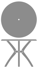
Arezzo Dining Table – 42" Round with Center Grommet, Wheelchair Height Model: ARG1W 42W 42D 31.75H
