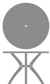
Arezzo Dining Table - 42" Round with Center Grommet, Standard Height Model: ARG1S 42W 42D 29.75H
