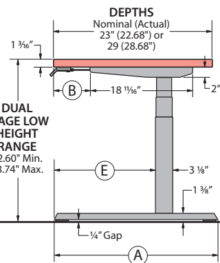
Side View (Dual Stage Low Option)
