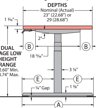
Side View (Dual Stage Low Option)
