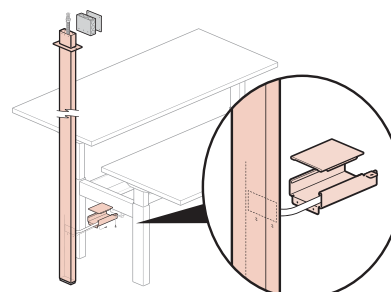
⑥ End of Run Top Feed
