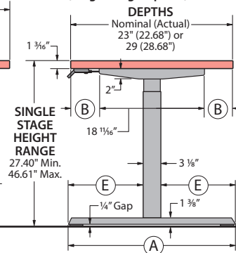
Side View (Single Stage Option)
