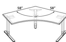
TLCZ-5858-NCEB C-Leg Corner, 120° Wrap-Around Electric Adjustment
