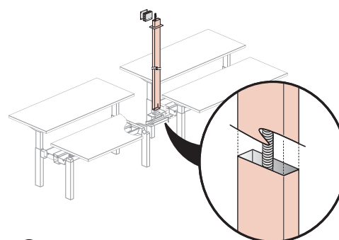
⑤ Middle of Run Top Feed
