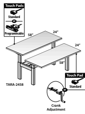
TARA-2458-NH Bench Crank and Electric Adjustment
