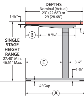
Side View (Single Stage Option)
