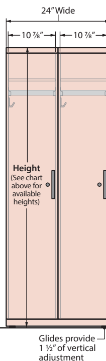
23 5/8" Deep Locker Front View
