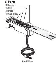
EWCG-3A3E-NPSCBNCW Narrow – Hardwire 6-Port
