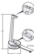
EUCN-PJ Collaborative Power Station
