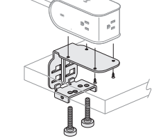
Standard Edge Worksurface Mount
