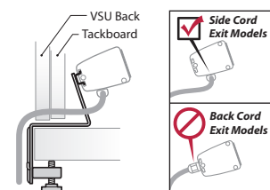
Side View Detail
