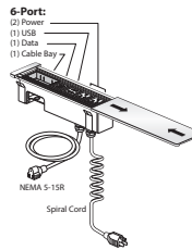
EWCG-3A3E-NPSCBNSF Spiral Corded – Height Adjustable 6-Port
