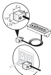
Circuit Breaker Plug Detail
