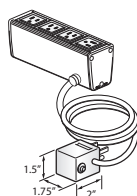
EUD1-PF0B-4000 6-Port Power Cord Circuit Breaker Plug
