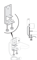
EUFB-0000-SB Classic Power Module Bracket - Vertical Bracket
