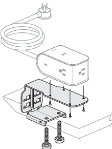
Knife Edge Worksurface Mount
