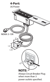
EWCG-4RNN-NPSCBNSL Corded – Height Adjustable 4-Port
