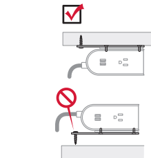
Above Worksurface Application (Bracket NOT Fastened or Needed)
