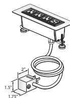
EUB1-PL0B-4000 4-Port Power Cord Circuit Breaker Plug
