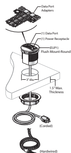
EUP1-PF0P EUP1-PJ0P EUP1-HF0P EUP1-HJ0P Flush Mounted Round
