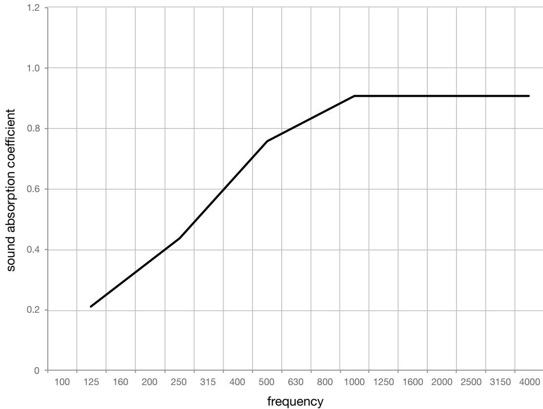
Soneo Floor Screen (NRC .75)
