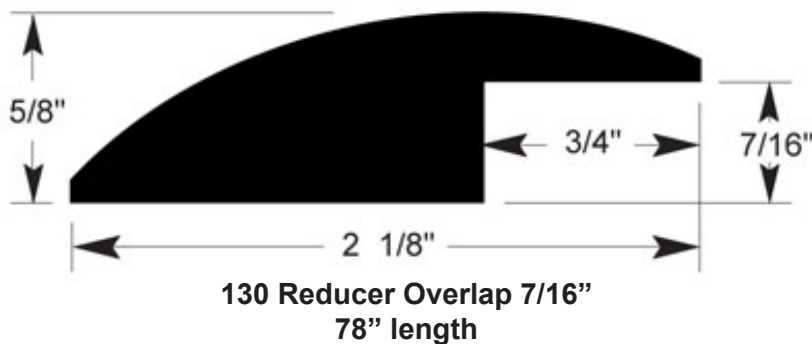
128 Threshold 7/16\" 78\" length
