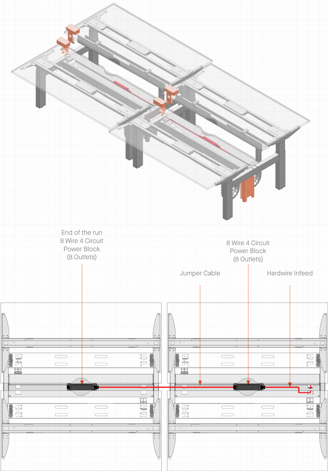
TYPICAL "H"-LEG DESK WIRING LAYOUT.
