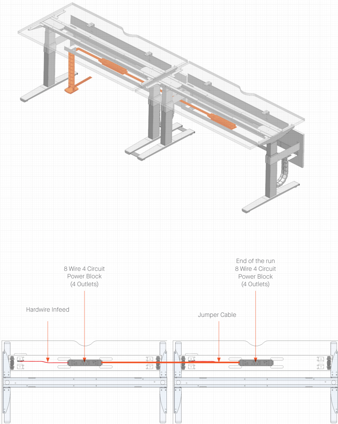
TYPICAL "I"-LEG DESK WIRING LAYOUT.
