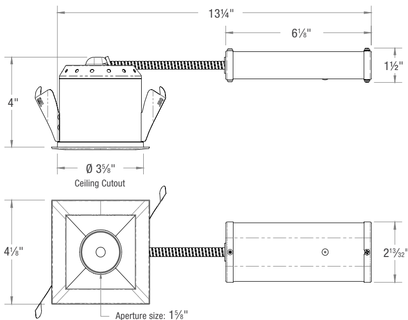
GSD-2 GYROSHIFT 2" SQUARE
