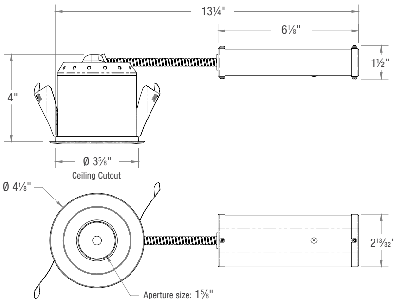
GSD-2 GYROSHIFT 2" ROUND
