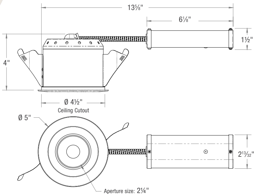
GSD-3 GYROSHIFT 3" ROUND
