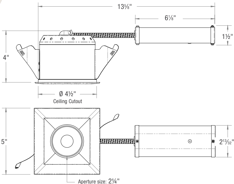
GSD-3 GYROSHIFT 3" SQUARE
