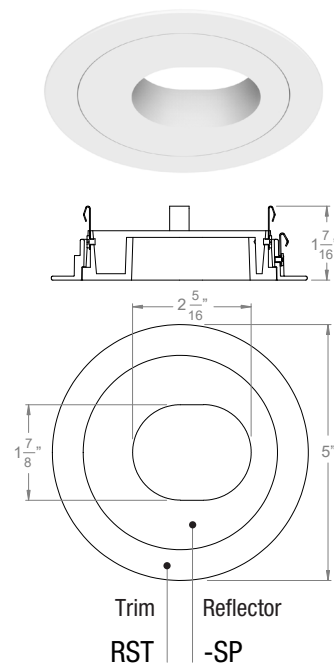
3" Acrobat Round Standard Trim with Slot Pinhole Reflector
