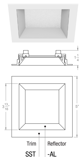
3" Acrobat Square Standard Trim with Adjustable Lensed Reflector
