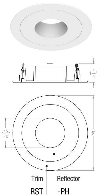
3" Acrobat Round Standard Trim with Pinhole Reflector
