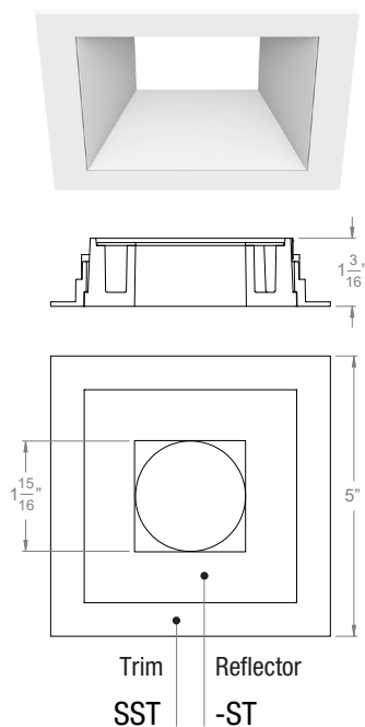
3" Acrobat Square Standard Trim with Standard Reflector
