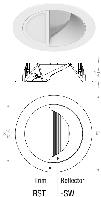
3" Acrobat Round Standard Trim with Wall Wash Reflector
