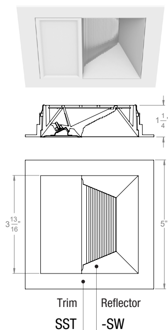
3" Acrobat Square Standard Trim with Wall Wash Reflector
