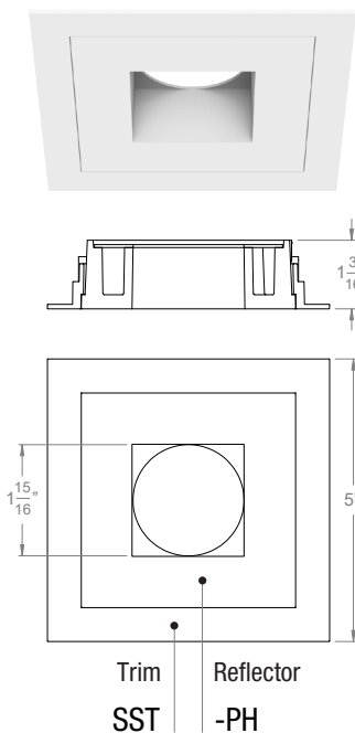
3" Acrobat Square Standard Trim with Pinhole Reflector
