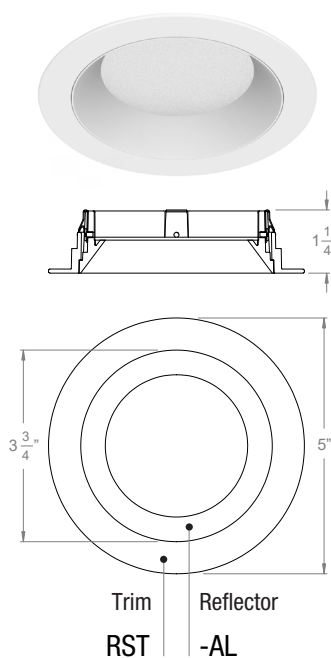
3" Acrobat Round Standard Trim with Adjustable Lensed Reflector
