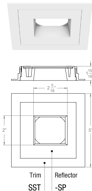
3" Acrobat Square Standard Trim with Slot Pinhole Reflector
