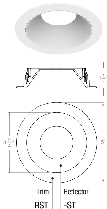
3" Acrobat Round Standard Trim with Standard Reflector
