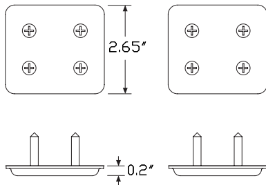
Desk & connecting bin ganging plates (C)
