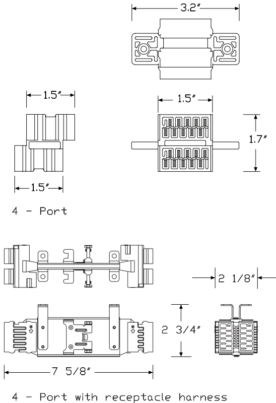
4 - Port with receptacle harness
