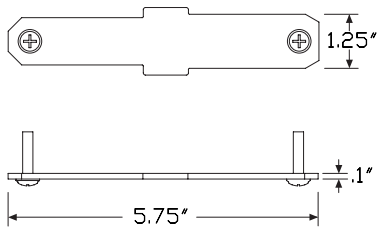
Peninsula table & freestanding bin ganging plates (B)
