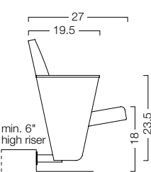
Riser Mount
