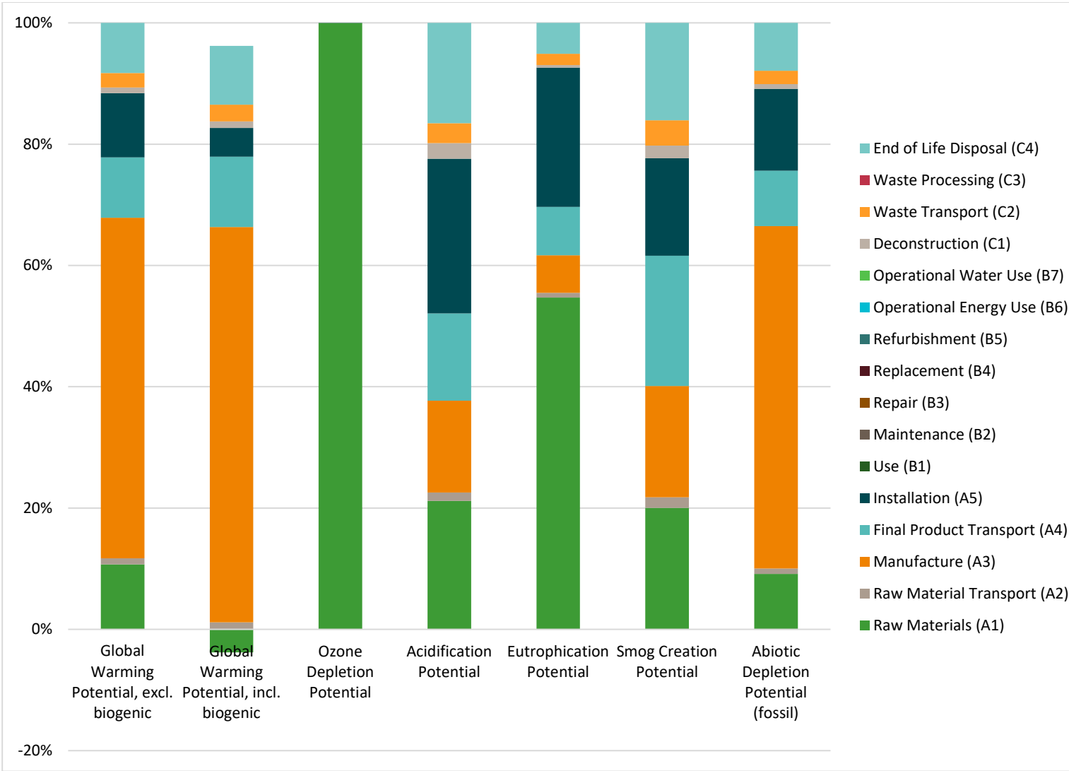
Figure 3: Cradle-to-Grave TRACI Environmental Impacts
