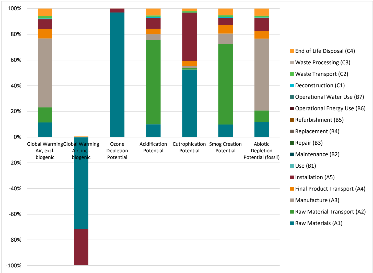
Figure 4: Cradle-to-Grave EN 15804 Environmental Impacts
