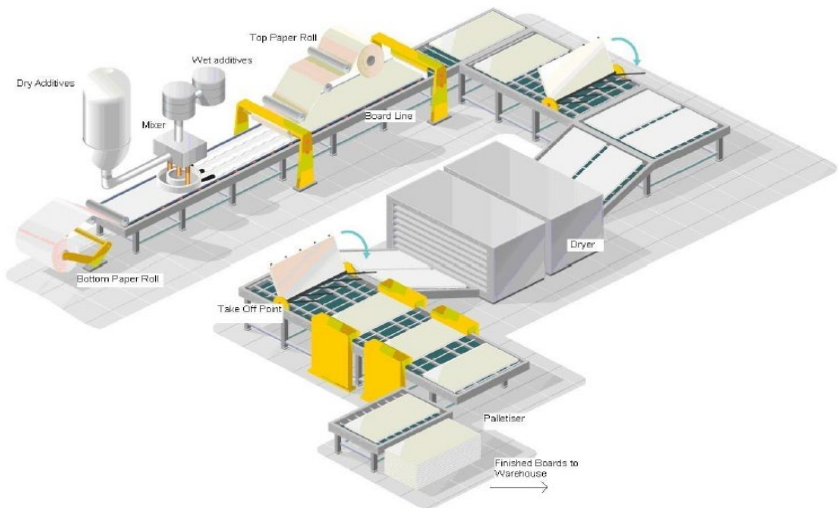
Figure 2: Gypsum Board Manufacturing Diagram
