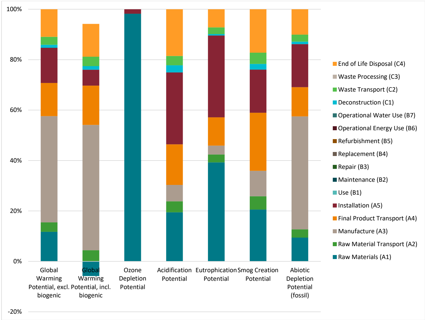
Figure 3: Cradle-to-Grave TRACI Environmental Impacts
