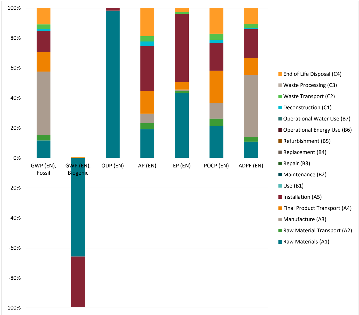
Figure 4: Cradle-to-Grave EN 15804 Environmental Impacts
