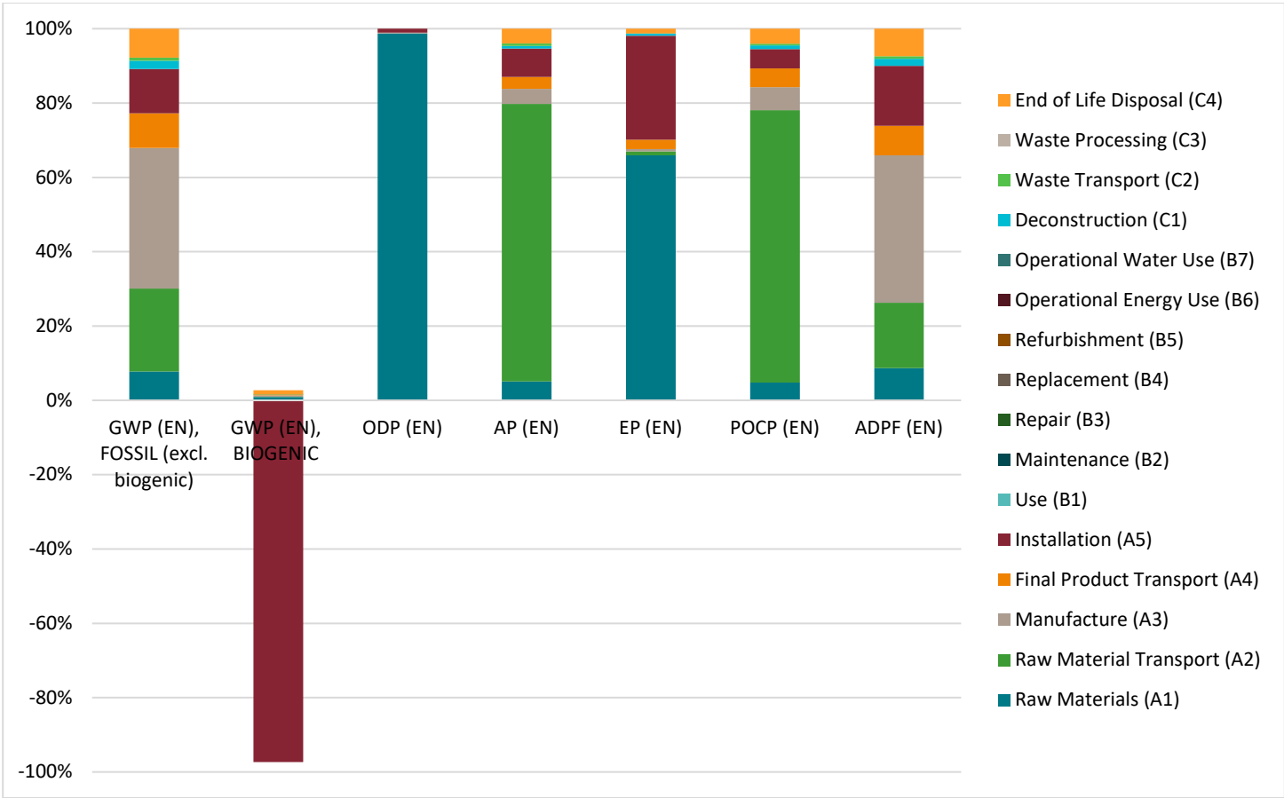
Figure 4: Cradle-to-Grave EN 15804 Environmental Impacts
