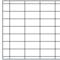
W-06 Pattern 3" x 1-1/2" rectangular opening Open area: 73%
