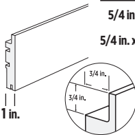
Built-in J-Pocket for siding
