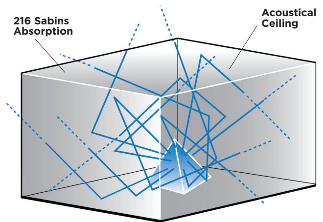
Figure 18: Acoustical ceiling adds 156 sabins, reduces noise level 5.5 dB.
