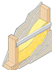
Steel 1 - STC 38 Standard construction
