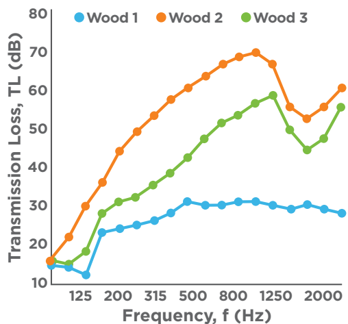
Wood 1 - STC 29 Standard construction
