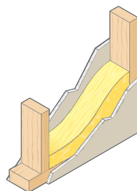
Figure 10: Conventional wood stud construction, single layer gypsum wallboard each side, 3-1/2" thick fiberglass insulation in wall cavity. STC: 39.
