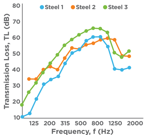
Steel 1 - STC 38 Standard construction
