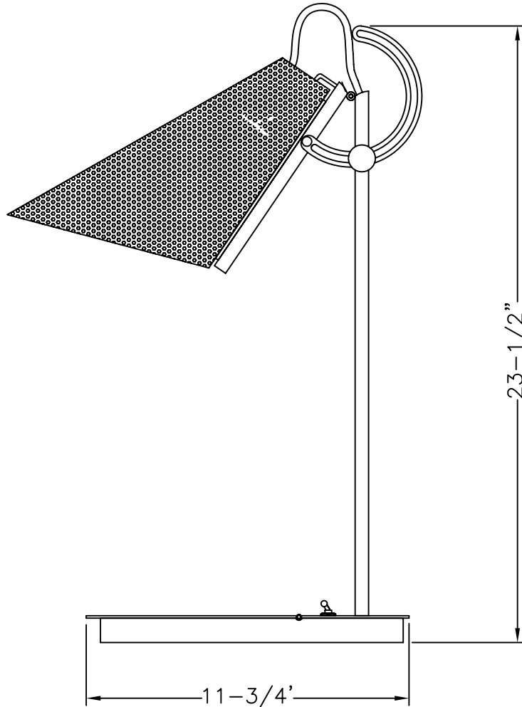
SIDE VIEW
