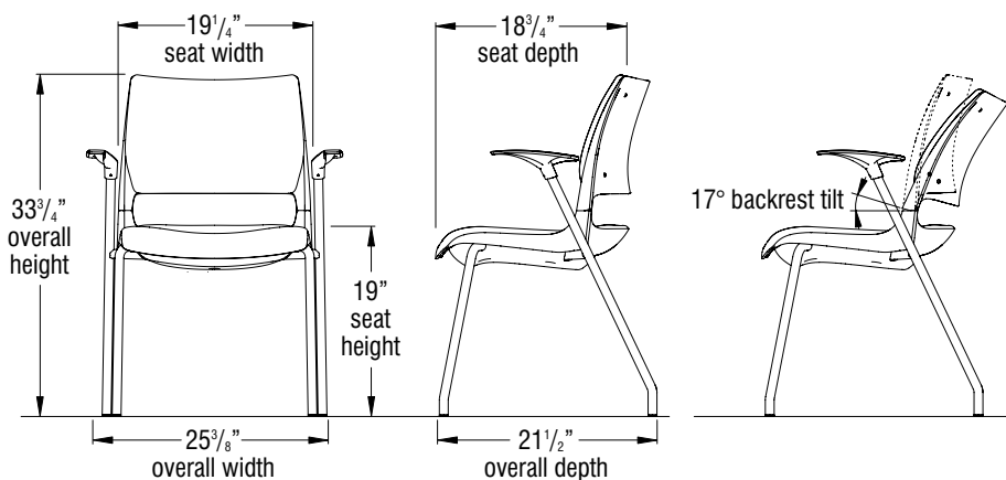
Doni 4-Leg Armchair
