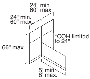
12" or 24" Glass stacker
