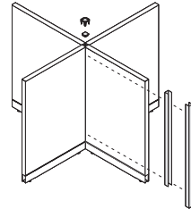
High X end cap or low universal end cap
