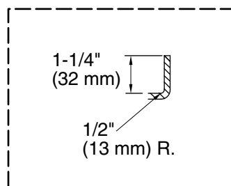
Integral Flange Detail
