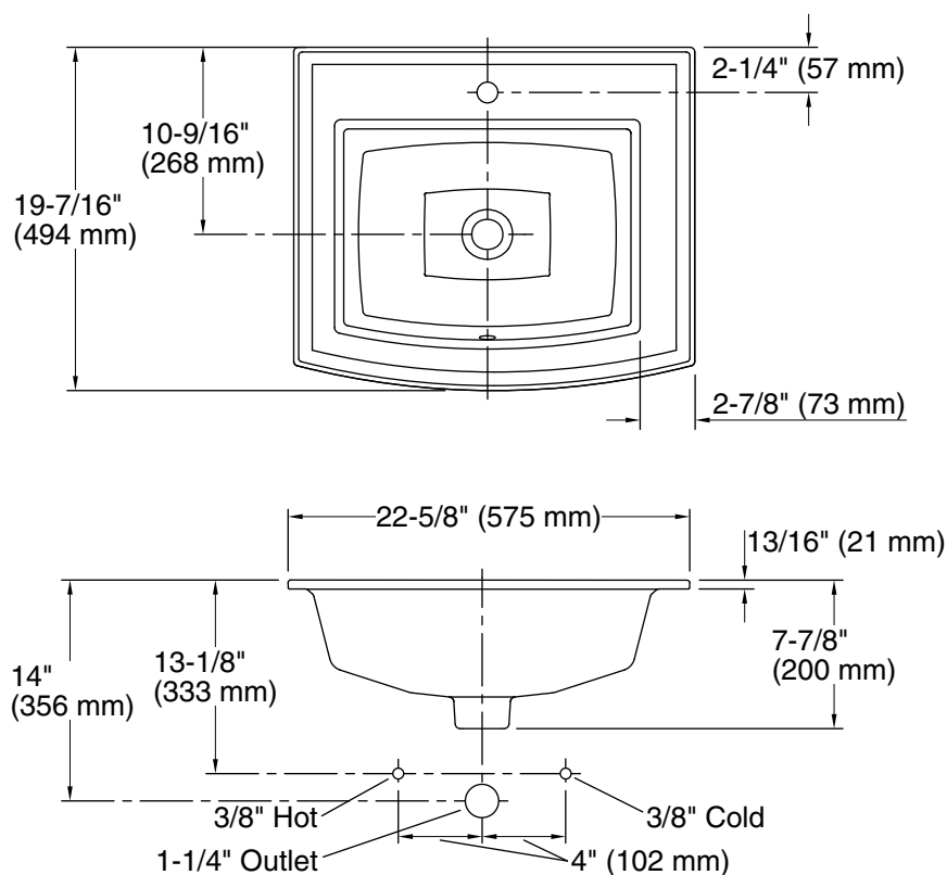
Standard Installation
