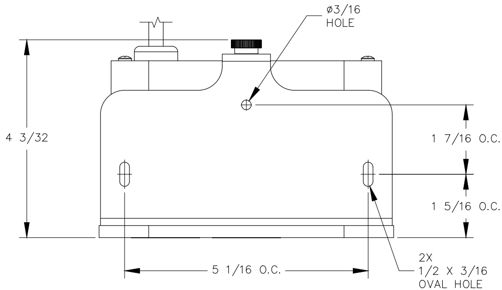
TOP VIEW
