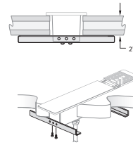
EWWM-0601 Flush Mount Power Module with Sliding Door Mounting Bracket for 2"(51mm) tops
