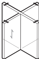
X Base 1.25" Thick 26", 32" Lengths
