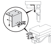
EUDB-0000 Mounting Bracket for Enhanced Power Modules
