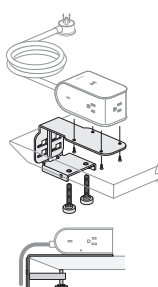
EUCB Knife Edge Worksurface Mount
