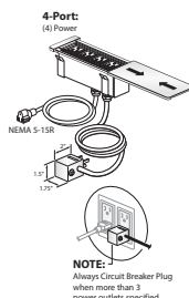
EWCG-4RNN-NPSCBNSL Corded – Height Adjustable 4-Port
