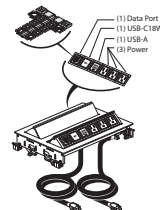
EUC2-PFOP-311010 Corded – Double-Sided
