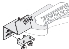
EUDB-0000-T Adjustable with Offset
