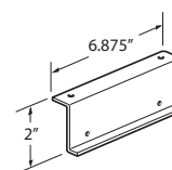
ZUAP-0000-PUR Under Surface
