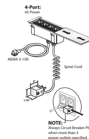
EWCG-4RNN-NPSCBNSF Spiral Corded – Height Adjustable 4-Port
