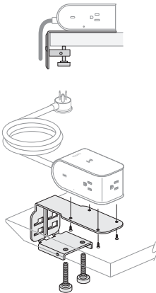
Knife Edge Worksurface Mount
