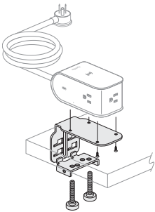
Standard Edge Worksurface Mount
