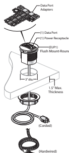
EUP1-PF EUP1-HF Flush Mounted Round
