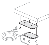
EUCB Under Worksurface Mount
