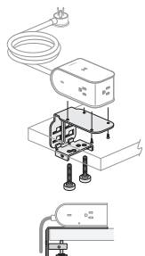
EUCB Standard Edge Worksurface Mount
