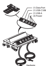
EUC2-HFOP-311010 Hardwire – Double-Sided
