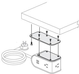
Under Worksurface Mount
