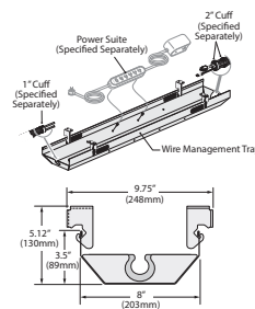
EUWT Wire Management Tray
