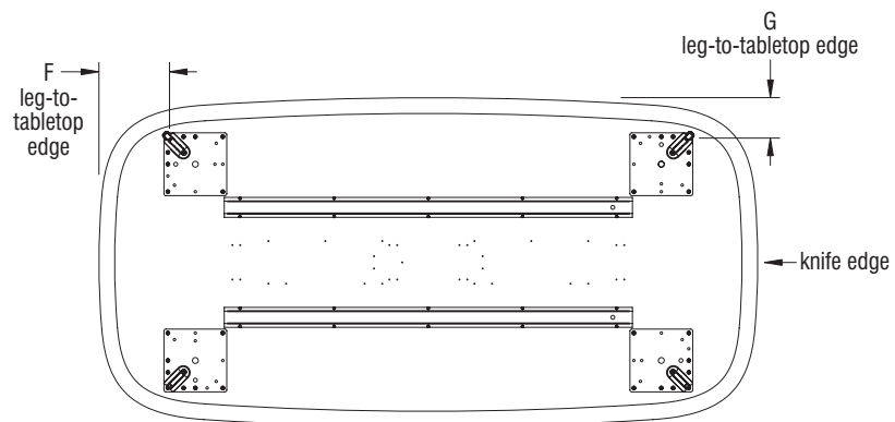
(bottom view)
