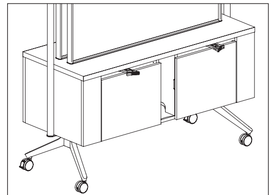
Cabinet Doors with No Locks - (ganging side)
