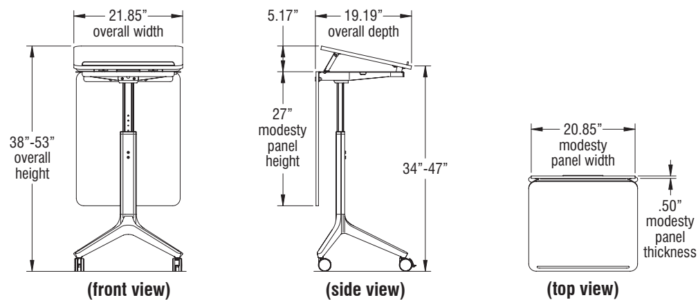
Tributaire Lectern, Screw-Adjustable Height
