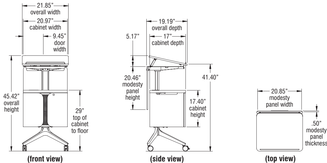
Tributaire Lectern with Storage, Screw-Adjustable Height
