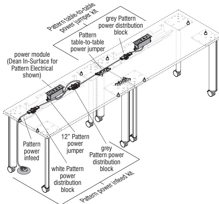
Tributaire Post-Leg Tables with Power Modules for Pattern Single-Circuit Electrical
