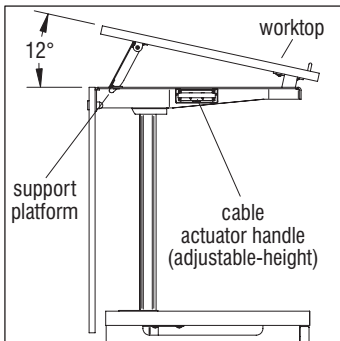
Worktop (raised 12°)
