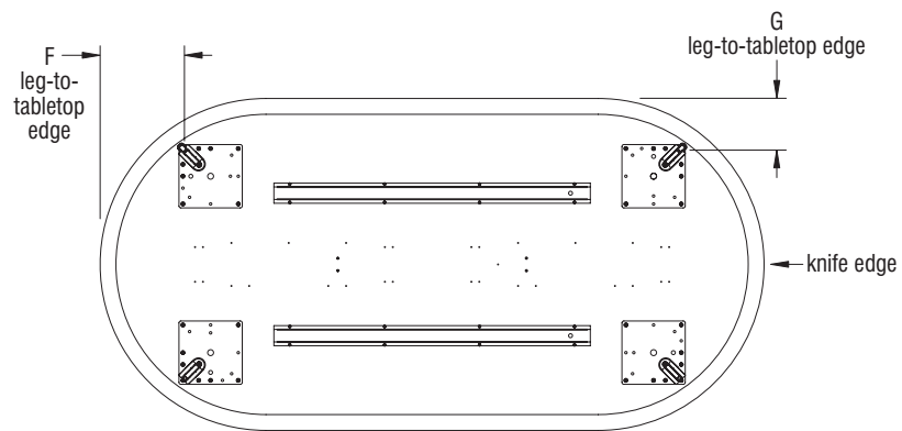
(bottom view)
