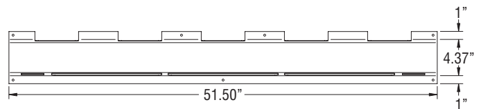
52" Wire Trough
