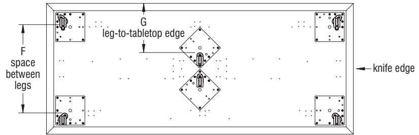
(bottom view)
