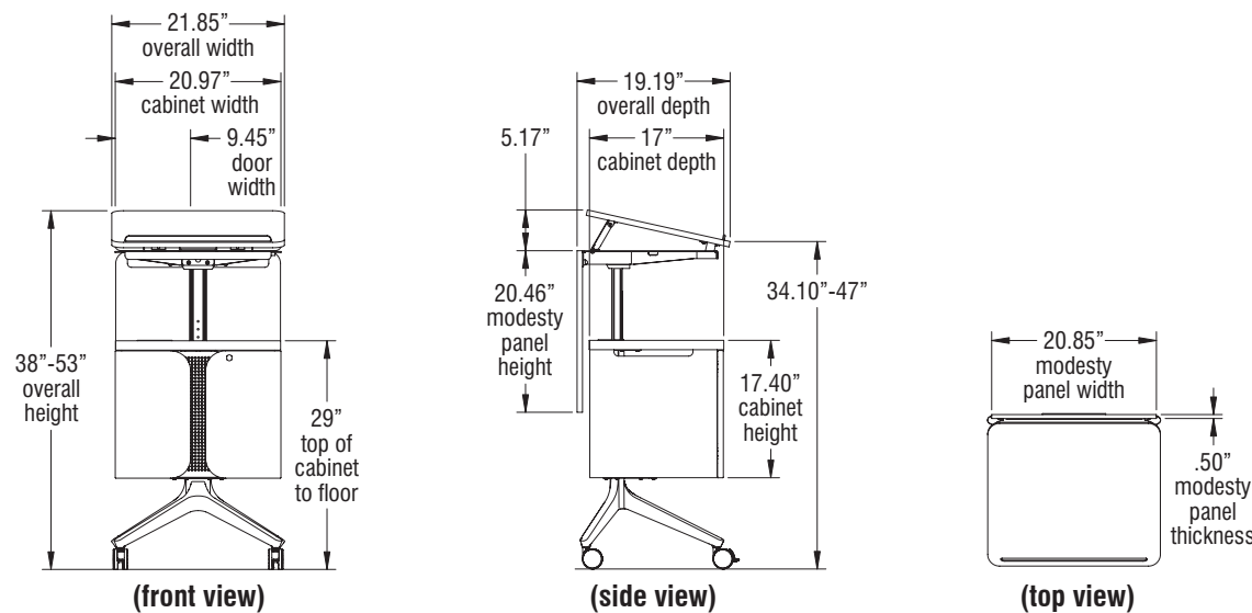
Tributaire Lectern with Storage, Screw-Adjustable Height
