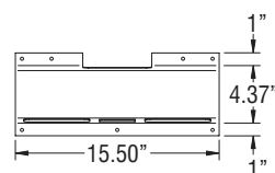
16" Wire Trough
