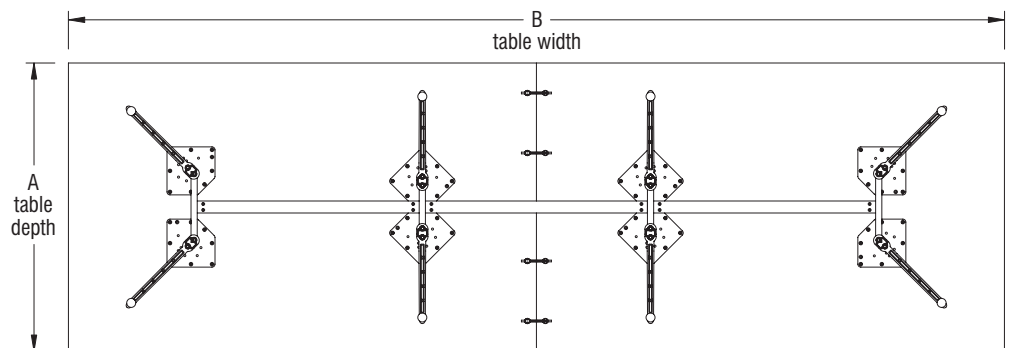
(bottom view)
