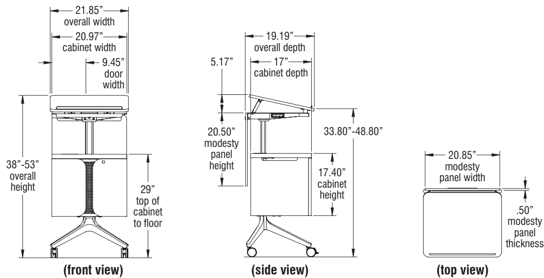
Tributaire Lectern with Storage, Pneumatic-Adjustable Height
