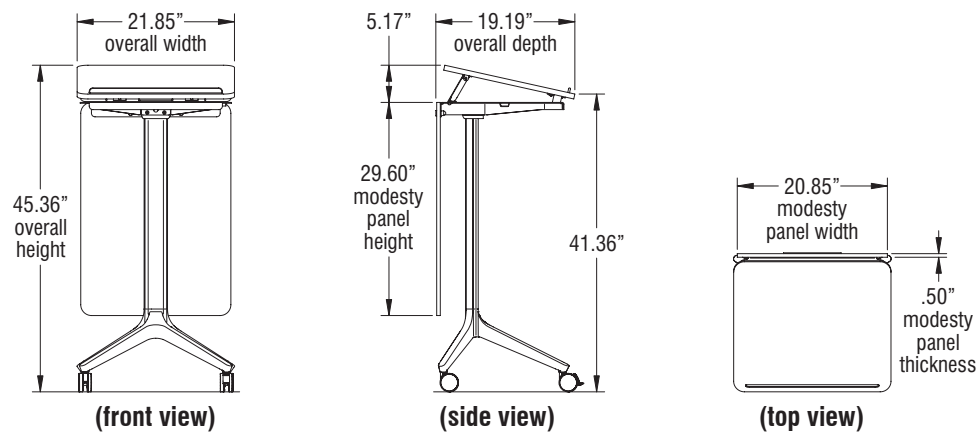
Tributaire Lectern, Screw-Adjustable Height
