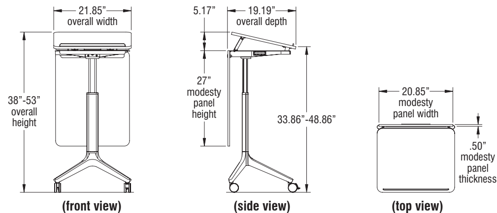
Tributaire Lectern, Pneumatic-Adjustable Height
