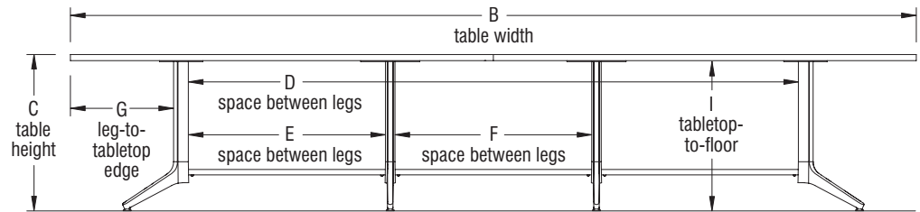
(front view)
