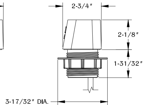
RIGHT VIEW
