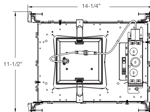
4" and 6" Square Frame (shown with 6" Light Engine)
