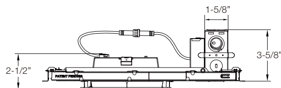
4" and 6" Square Frame (shown with 6" Light Engine)
