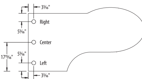
Extended P/U Shaped Worksurface (Right shown)
