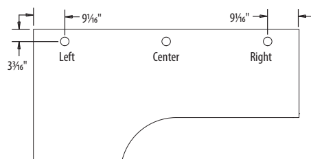
Extended Corner Worksurface (Right shown)
