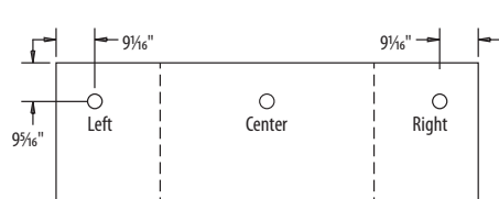
30" and 36" deep Worksurfaces
