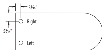
U-Shaped Desk
