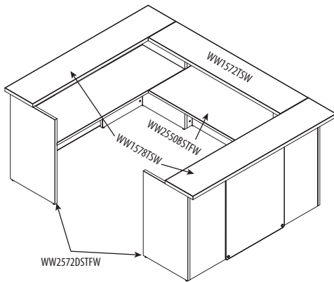
Fig. G – 2 Main Shells with Reception Bridge (Counters across entire unit)
