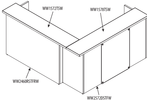
Fig. C – Main Shell with Reception Return (Counters across entire unit)
