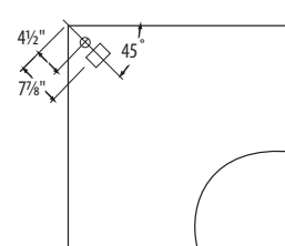
Corner Worksurface
