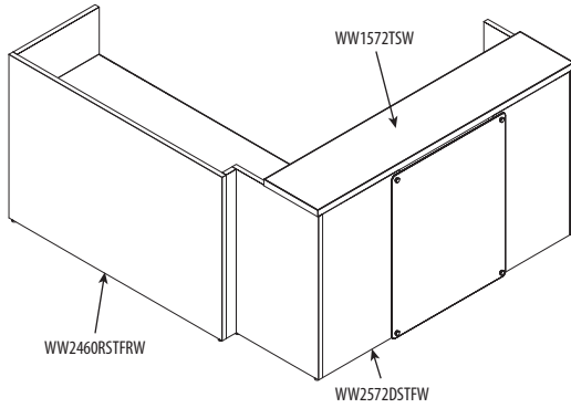
Fig. A – Main Shell with Reception Return (Counter on main shell)
