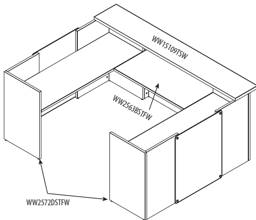
Fig. E – 2 Main Shells with Reception Bridge (Counter on reception bridge spanning main shells)
