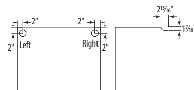
End Panel
