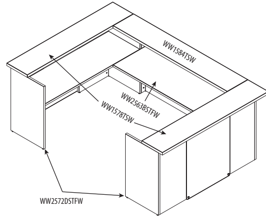
Fig. H – 2 Main Shells with Reception Bridge (Counters across entire unit)
