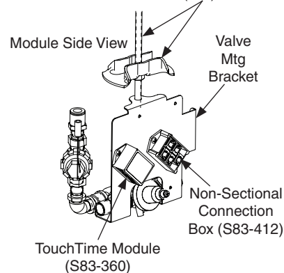
Module Side View Tie Rod and Tie Bar (Ref)
