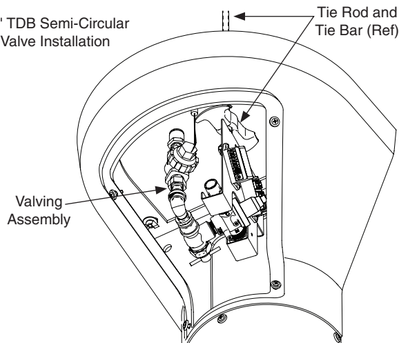
Valve Side View Tie Rod and Tie Bar (Ref)
